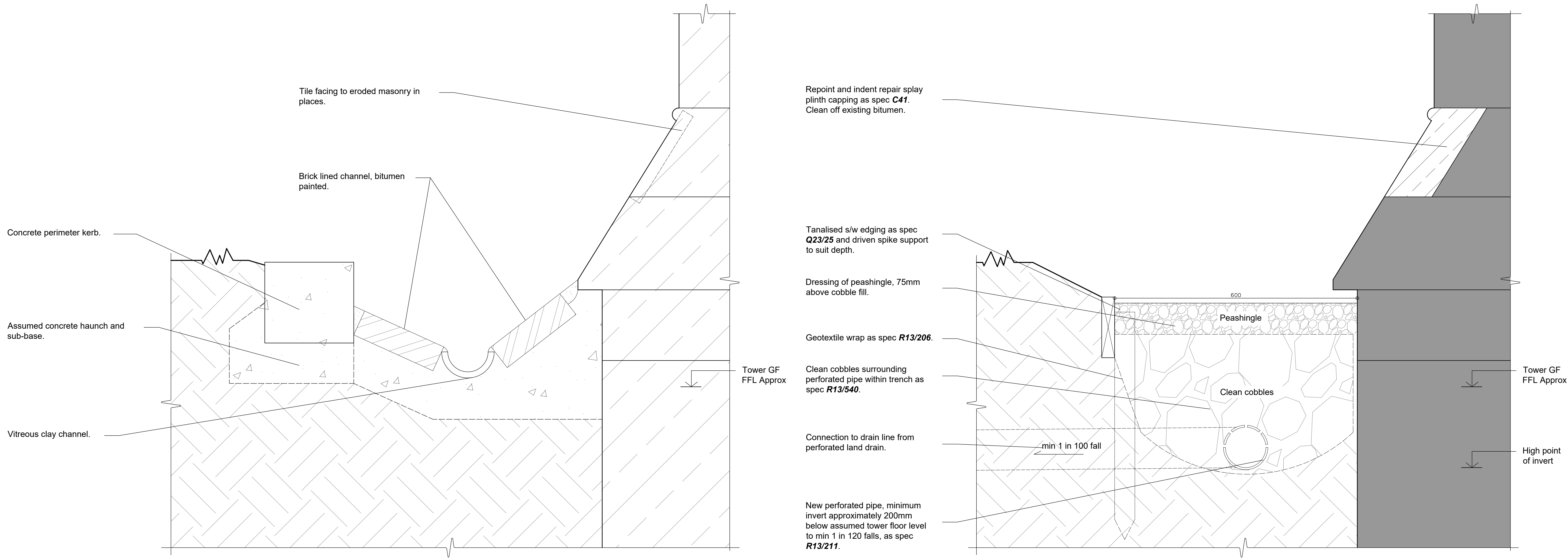
1 Existing Assumed Trench Construction at Tower Scale: 1:5
