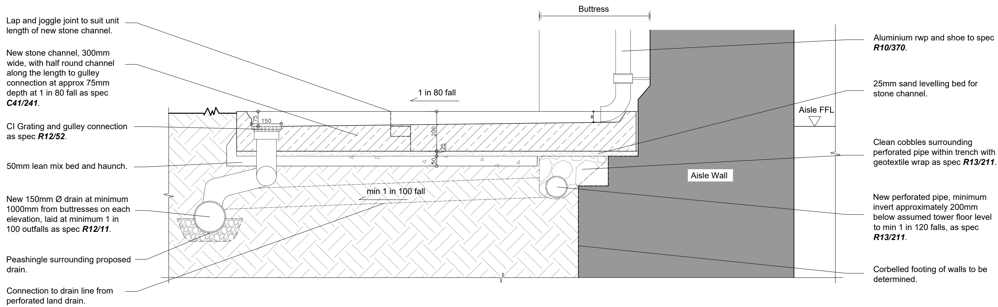
3 Proposed Outfall to Rainwater Pipes Scale: 1:5
